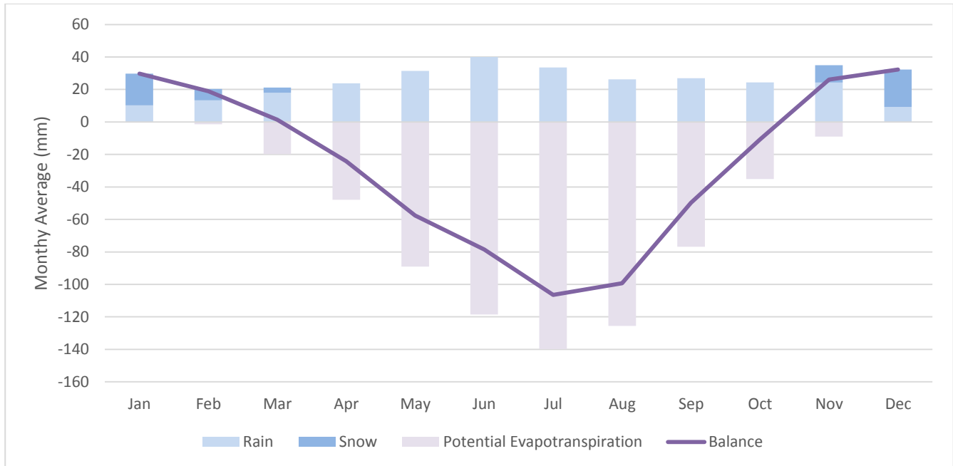
Figure 3: West Kelowna Climate Data (PC Burnett's Nursery)
