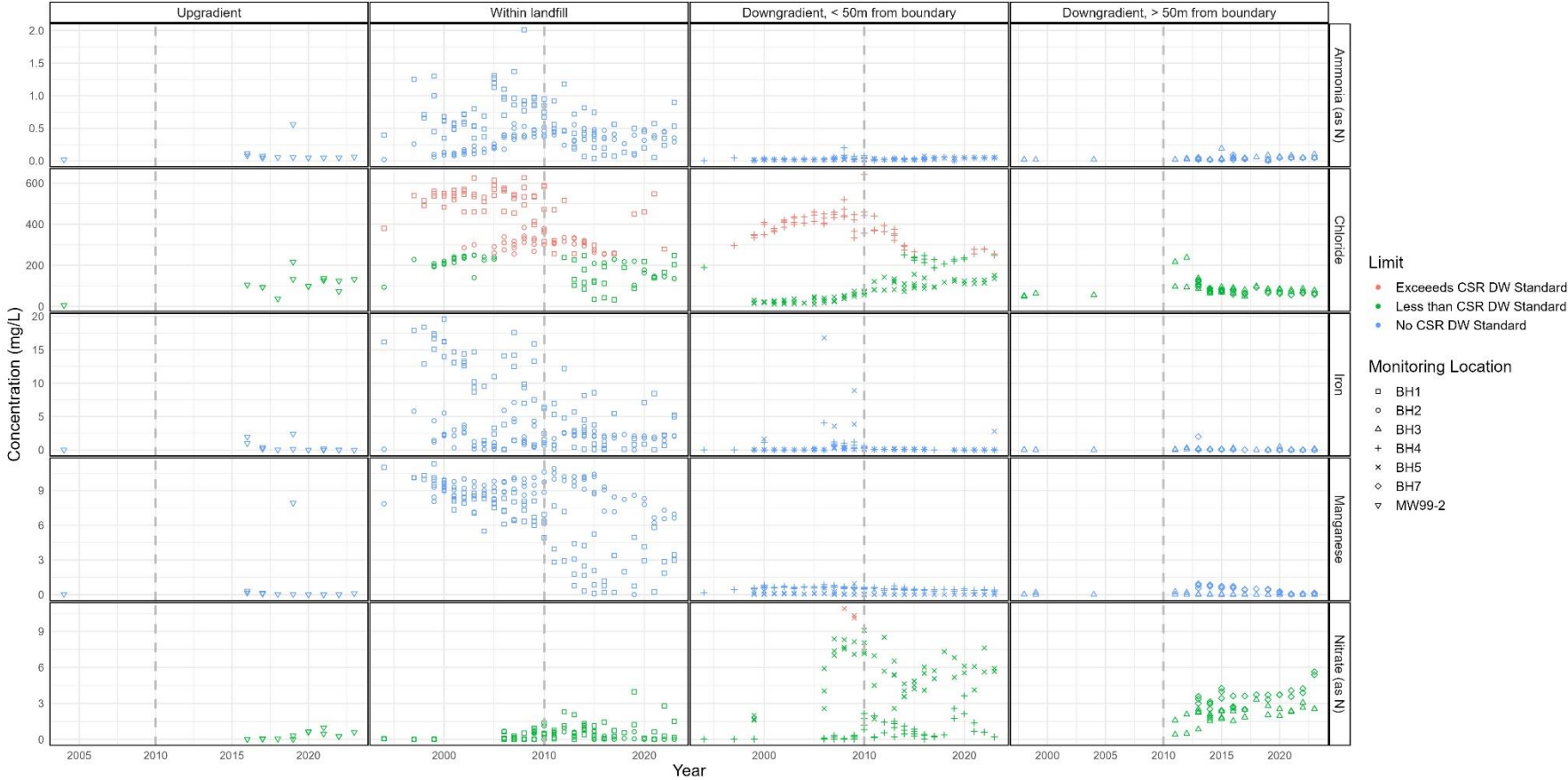
Figure 6: Values of Key Parameters in Groundwater Over Time
