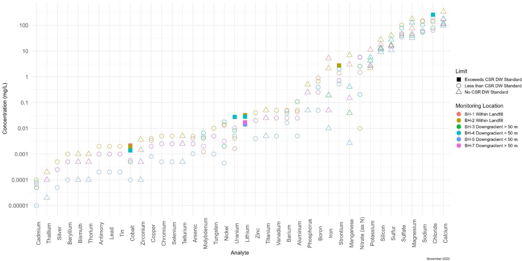
Figure 5: Groundwater Quality Summary, November 2023
