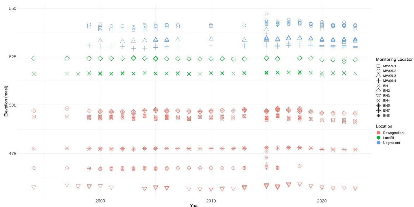
Figure 8: Groundwater Elevations, by Well
