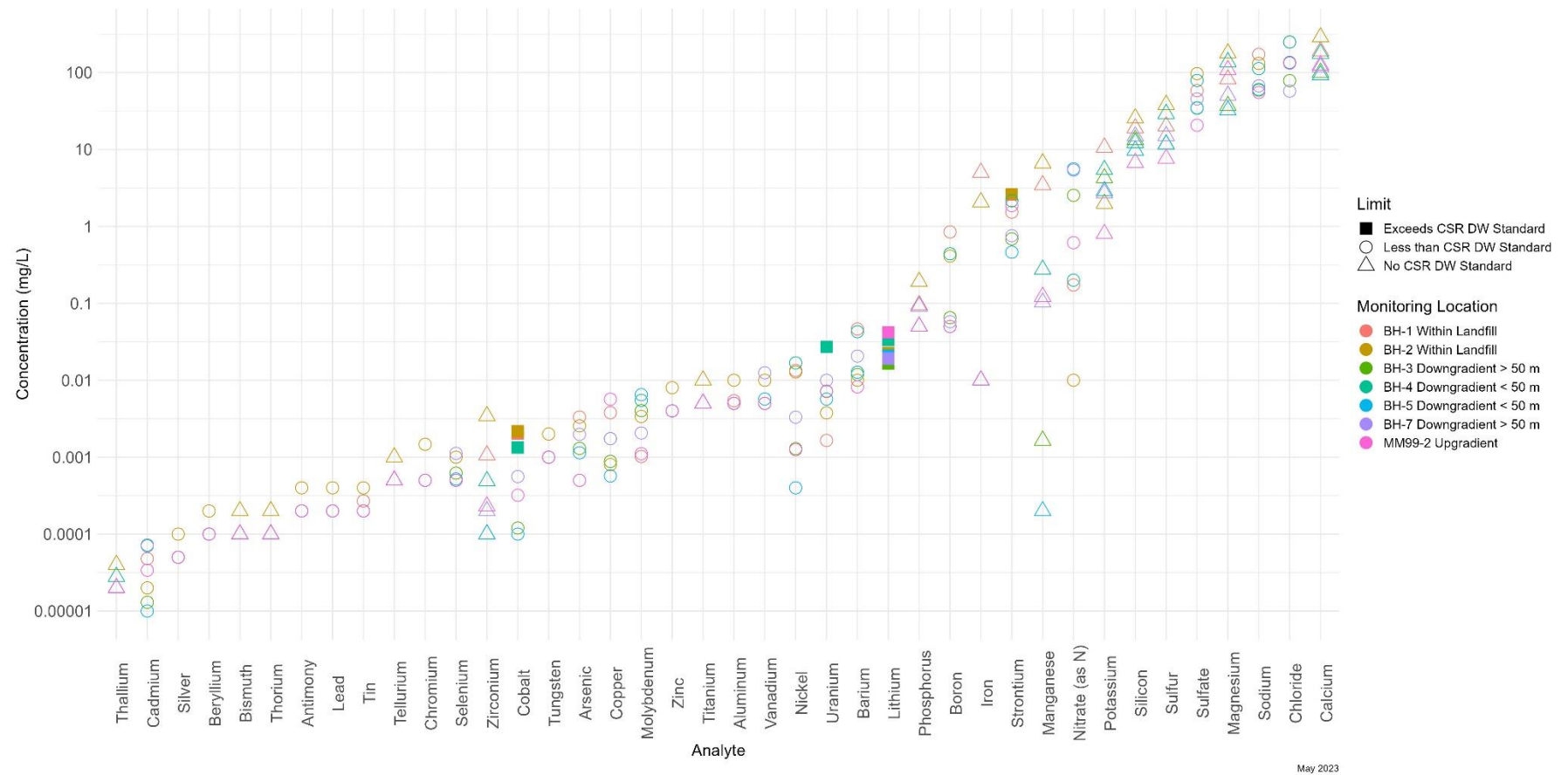
Figure 4: Groundwater Quality Summary, May 2023
