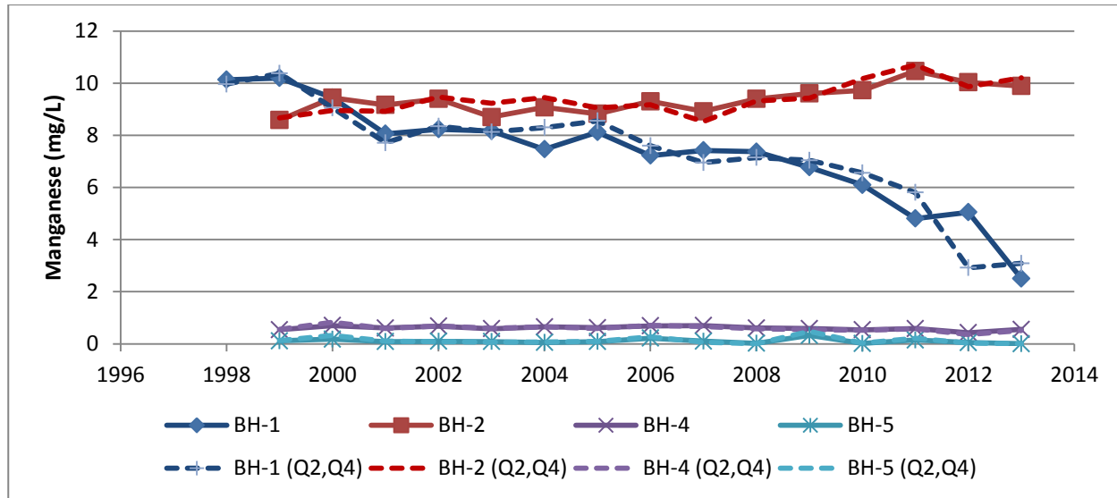
Figure 15: Manganese - Average Concentration based on Annual and Q2 plus Q4 results
